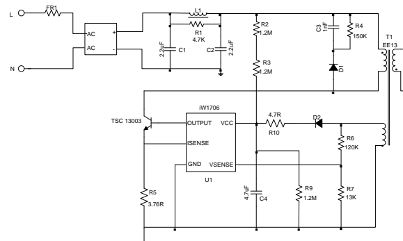
Figure 2 Based on iW1706 LED driver power supply circuit
