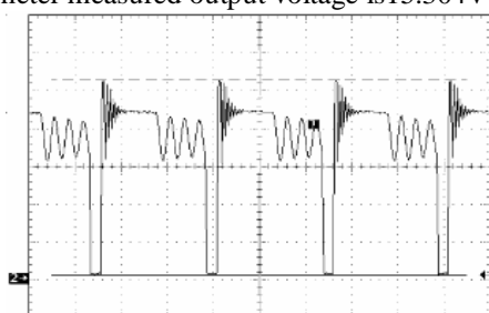
(a) Vce wave form switch
