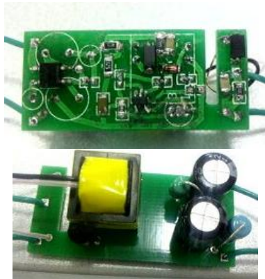
Figure3 Switching power supply design physical map (bottom left,top right picture)
