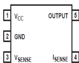
Figure 1 iW1706's pinout
